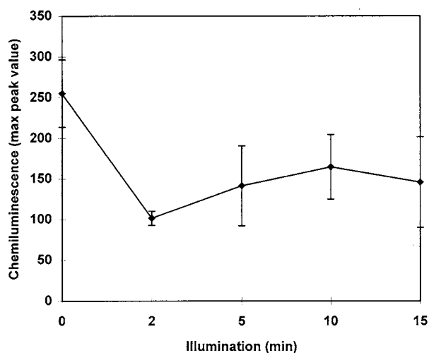
Fig. 2. Time response effect of illumination with SOE on isoluminol amplified chemiluminescence in PMA-activated human monocytes. Monocytes ( 5 \times 10^5 cells) were incubated for different times at 37^\circ\text{C} with or without SOE, mixed with 56\text{-}\mu\text{M} isoluminol in KRG and 4 units HRP. Then PMA ( 10\text{-nM} final concentration) was added and the light emission was recorded for 15 min. The results of 2-, 5-, and 10-min illumination are the mean \pm SEM of five experiments, and the result of 15-min illumination are the mean \pm range of two experiments, each conducted with monocytes from different donors. The values represent maximal peak values of chemiluminescence \text{mV}/5 \times 10^5 cells.
