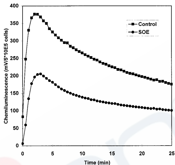
Fig. 1. Effect of singlet oxygen energy (SOE) on chemiluminescence from monocytes induced by PMA 10 nM. Monocytes ( 5 \times 10^5 cells) were incubated for 10 min at 37°C with or without SOE, mixed with 56- \mu M isoluminol in KRG and 4-units HRP. Then PMA (10 nM final concentration) was added and the light emission was recorded for 25 min. Representative curves are shown from monocytes exposed to SOE (●) and control cells not exposed to SOE (■).
