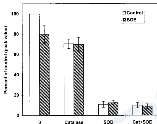
Fig. 3. Effect of catalase and SOD on treatment with SOE on PMA-induced chemiluminescence in monocytes. Monocytes ( 5 \times 10^5 cells) were incubated for 10 min at 37^\circ\text{C} with or without SOE (air treatment), mixed with 56\text{-}\mu\text{M} isoluminol in KRG and 4-units HRP with and without catalase 2000\text{ U/ml} and SOD 50\text{ U/ml} . Then PMA ( 10\text{-nM} final concentration) was added and the light emission was recorded for 15 min. The results are the mean \pm SEM of six experiments each conducted with monocytes from different donors. The values represent percent of control maximal chemiluminescence peak values.
